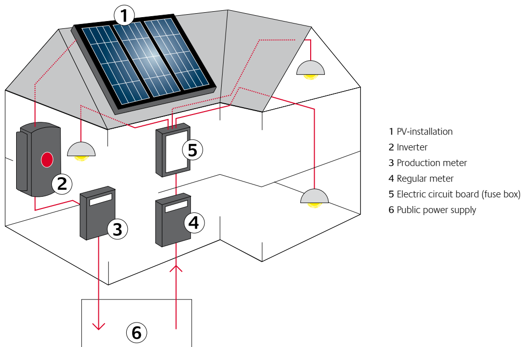
Layout and functionality of a grid-connected photovoltaic system
