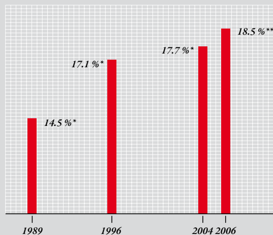
Efficiency of square polycrystalline solar cells: *15 x 15 cm, ** 15 x 15.5 cm
