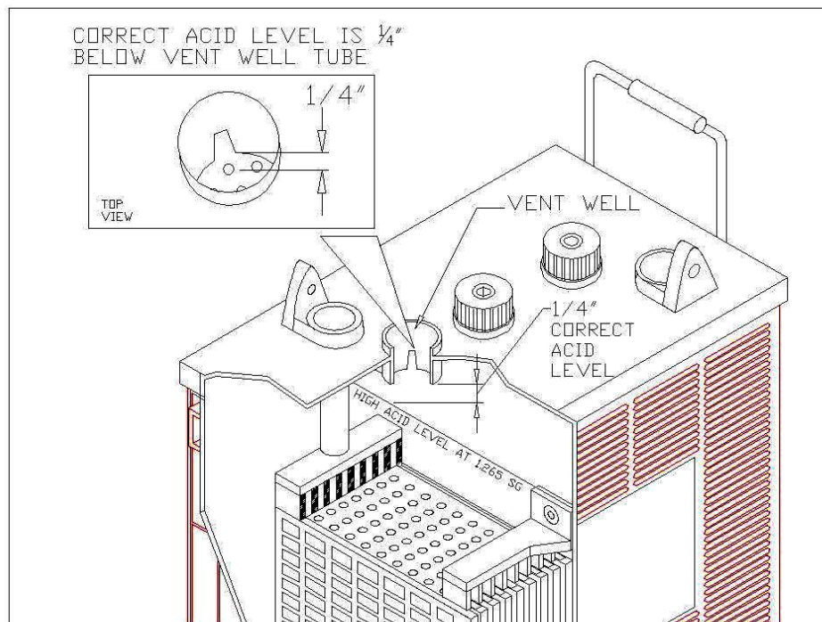
Figure 4, Electrolyte level
