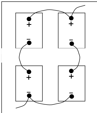
Figure 3 - Voltage/Capacity Increase
