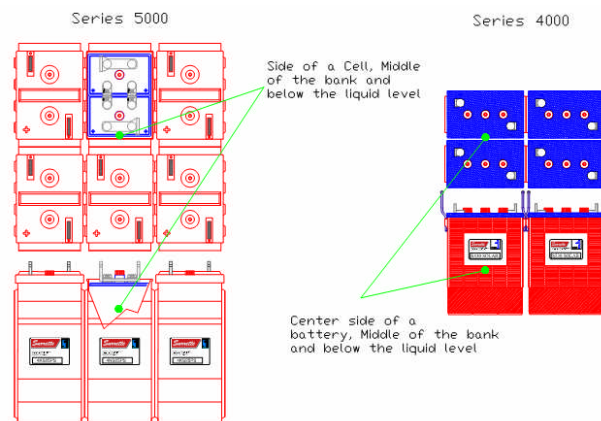
Figure 2, Temperature Probe
